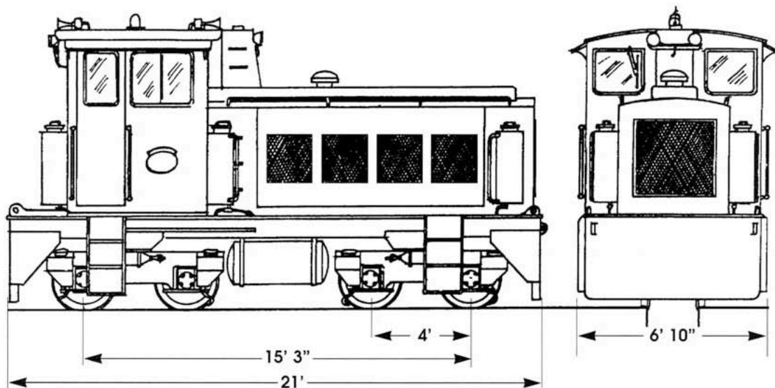
NAMBOUR SUGAR MILLS 18 TON E. M. BALWIN BOGIE DIESEL LOCOMOTIVE. 2' Gauge
